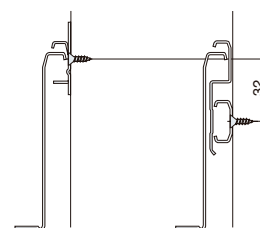
TELESCOPIC "GACELA" RUNNER
