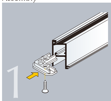
FIXED TRAY
