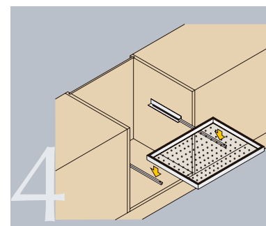
PULL-OUT TRAY
